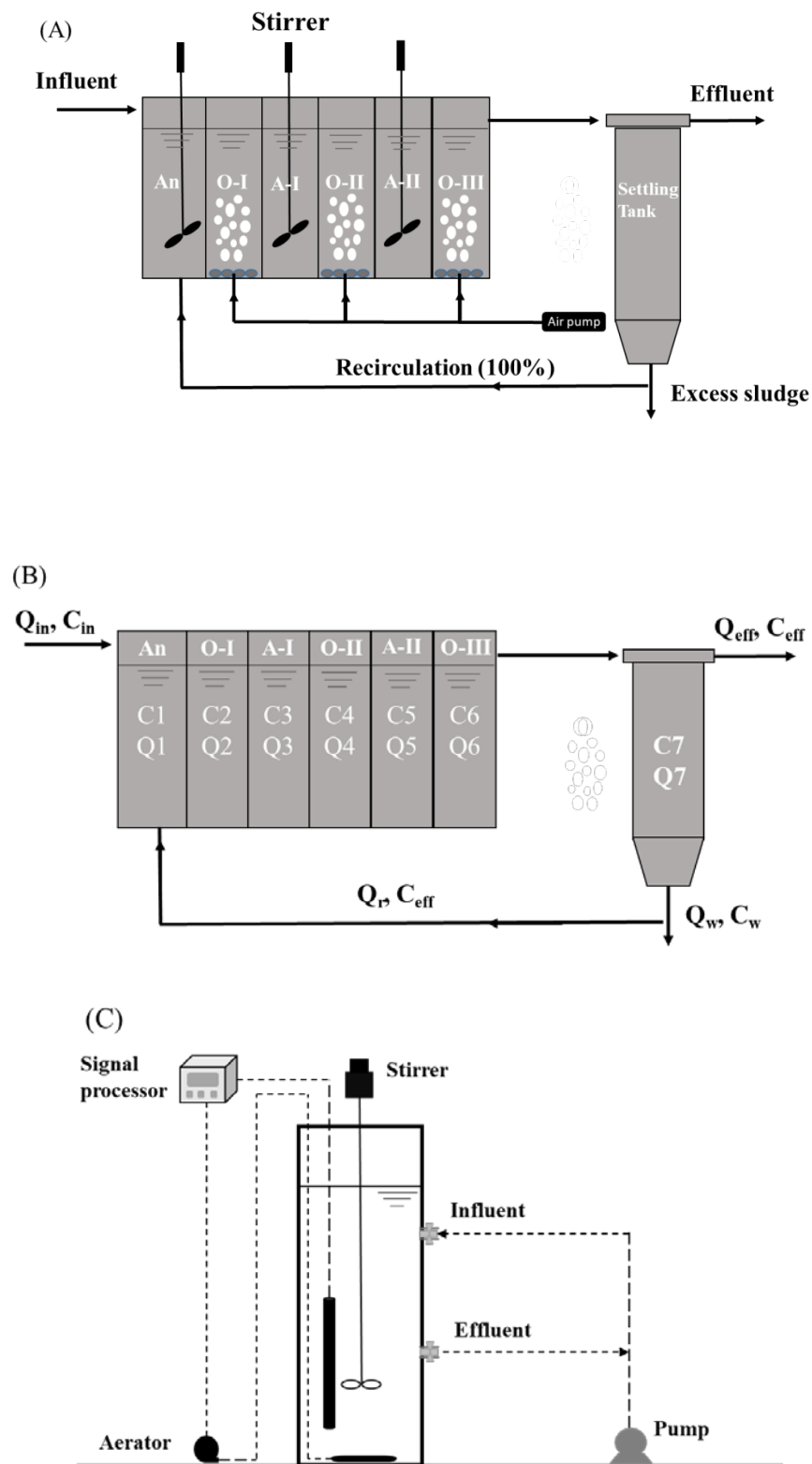
Fig. S1. Configuration of SBR (A) and CMR (C) system; schematic diagram of nitrogen and phosphate balance (B). An, A and O represent anaerobic, anoxic and aerobic tank, respectively.
