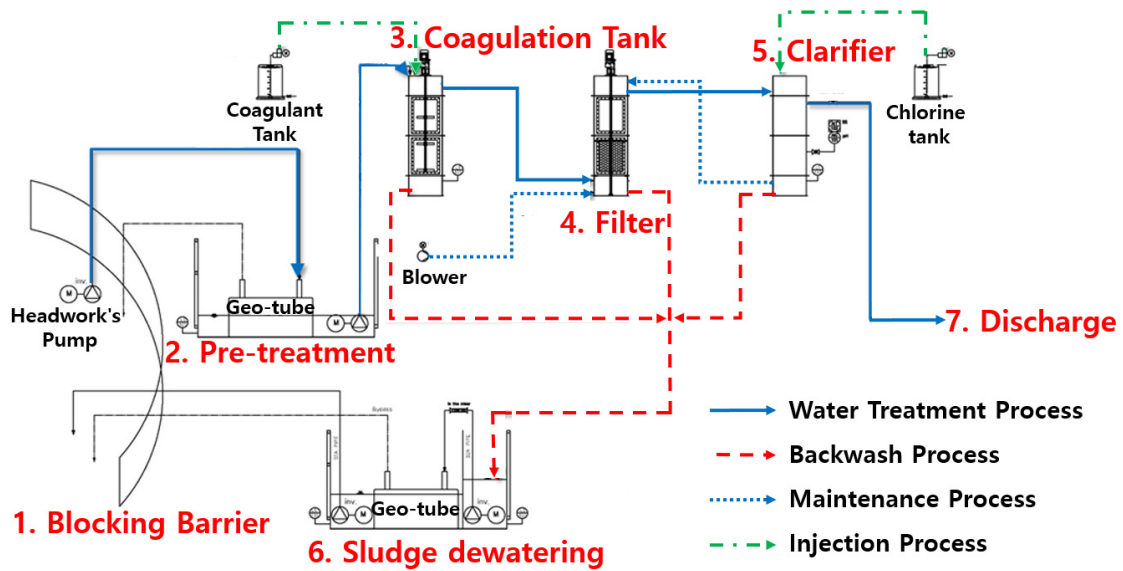
Fig. S3. Schematic diagram for the movable treatment unit
