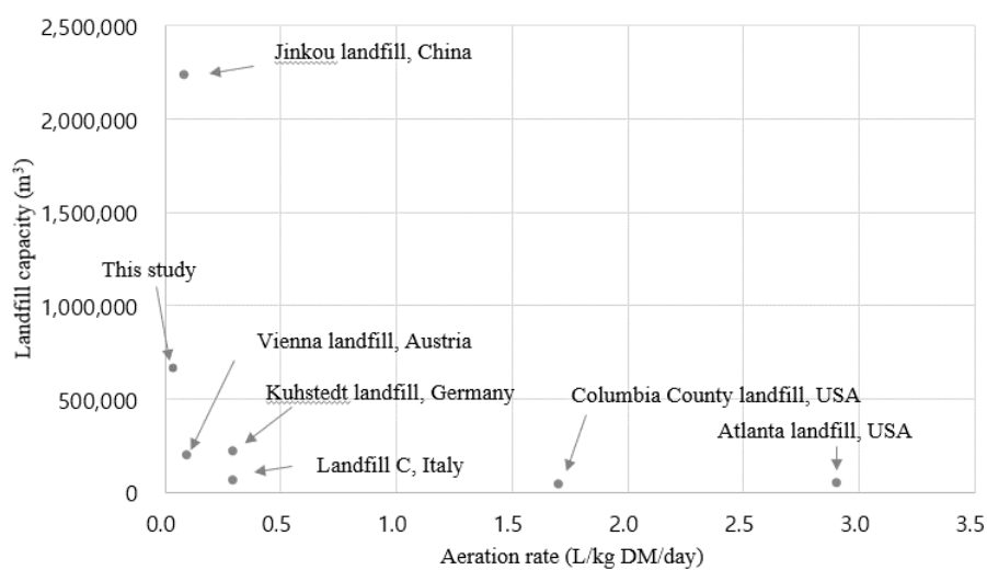
Fig. S2. Aeration rates in different aerobic landfills
