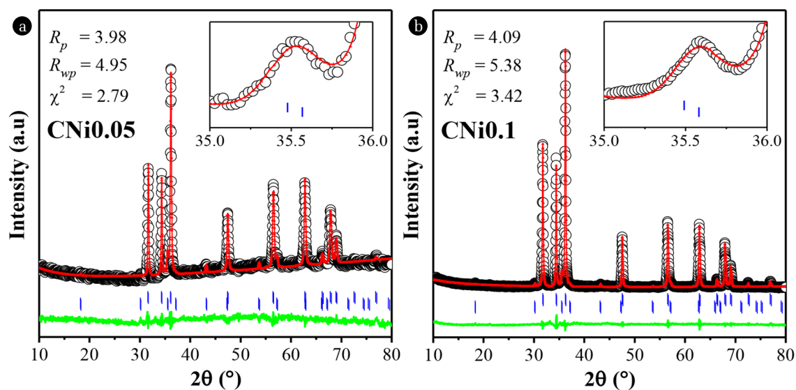
Fig. S1. Le Bail refinement plot of the composite CNi0.05 and CNi0.1 samples using the multiphase refinement system of ZnO and NiFe 2 O 4 . The presence of the NiFe 2 O 4 phase was determined by the Bragg reflection of each phase following the XRD peaks in the inset figure.
