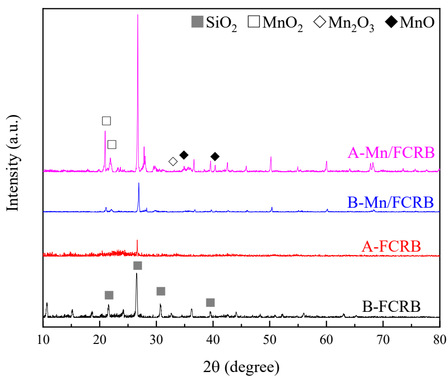
Fig. S1. XRD spectra of the Mn/FCRB.
