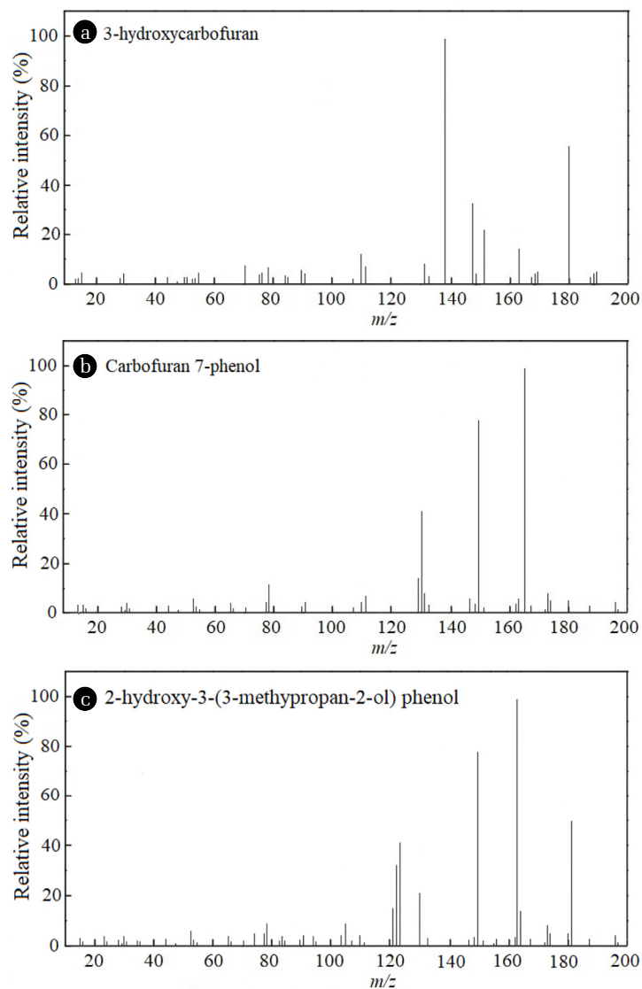
Fig. S1. GC/MS of some intermediates in degradation of carbofuran by Bacillus sp. strain DT1; (a) 3-hydroxycarbofuran, (b) carbofuran 7-phenol and (c) 2-hydroxy-3-(3-methypropan-2-ol) phenol.
