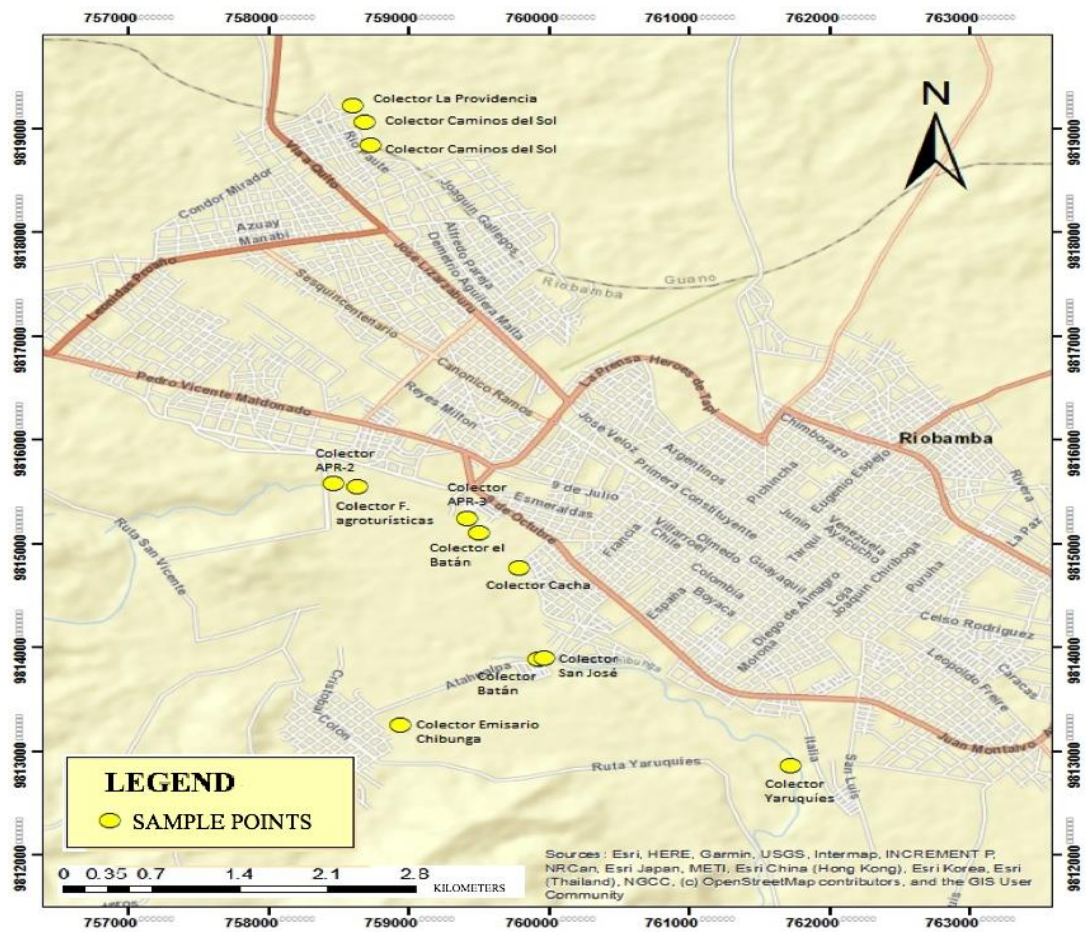
Fig. S1. Map of sampling points for microplastic analysis.
