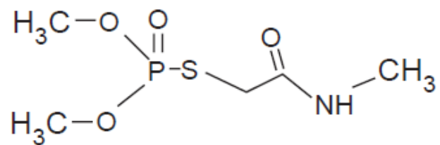
Fig. S1. The chemical structure of omethoate.
