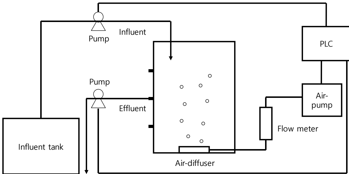
Fig. S1. Schematic diagram of lab scale reactor.
