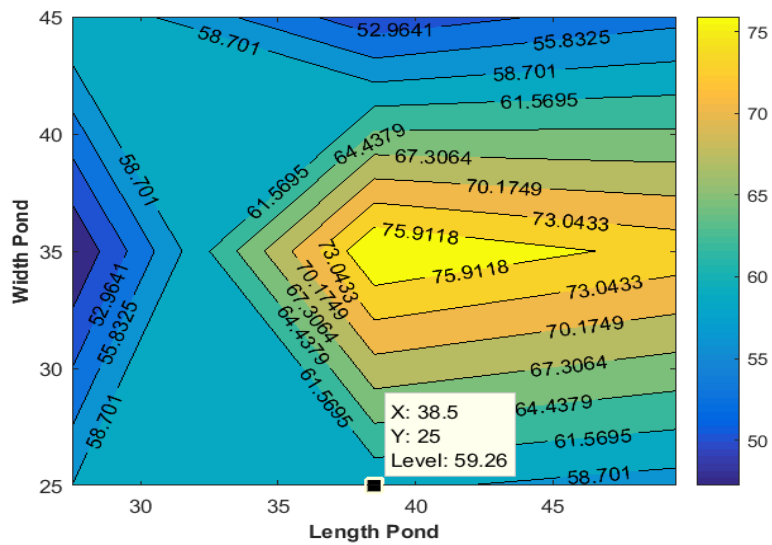
Fig. S4. Distribution of BOD on Pond Depth of 1 meter at t = 6 h.
