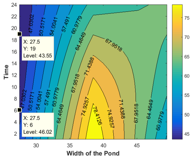
Fig. S1. Distribution of BOD on the width side of the pond.
