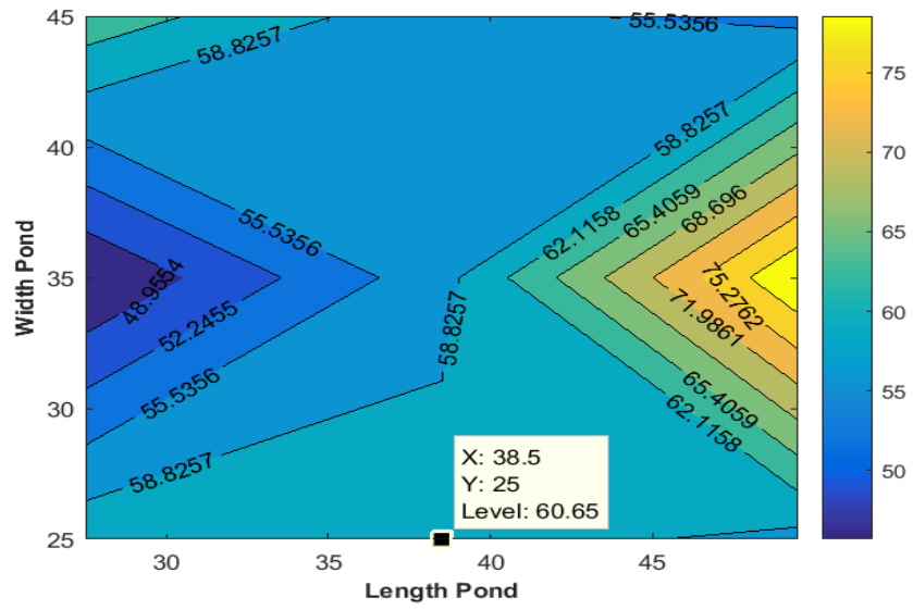
Fig. S5. Distribution of BOD on Pond Depth of 1 meter at t = 19 h.
