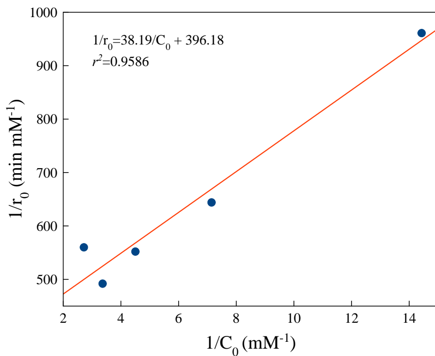
Fig. S1. Linear plot for Langmuir-Hinshelwood-Hougen-Watson (LHHW) kinetic model.
