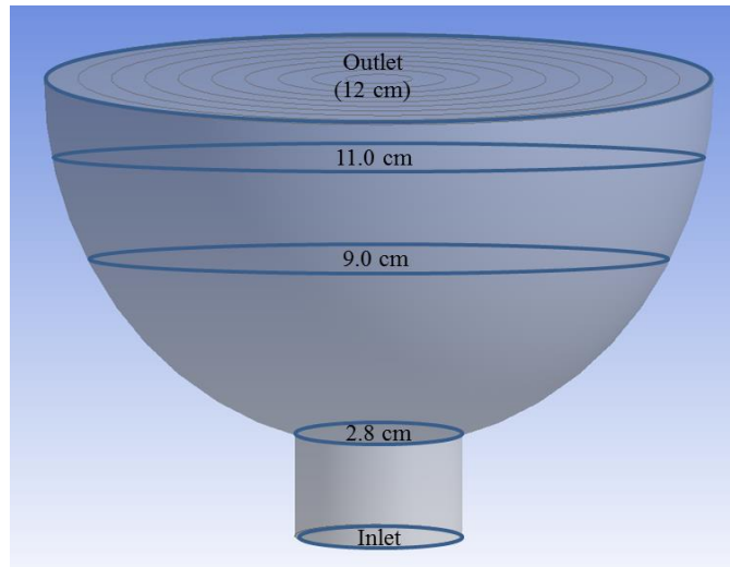
Fig. S1. Locations used to measure the non-uniformity coefficient and energy utilization.
