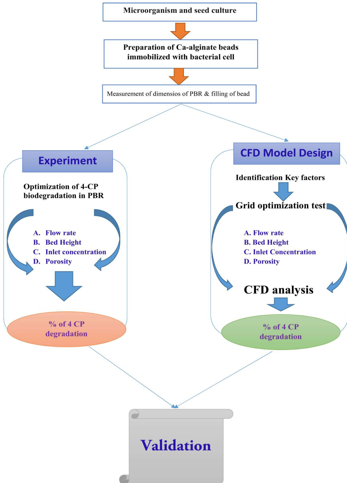
Fig. S1. Process flowchart of 4-CP degradation in immobilized catalysed packed bed reactor.
