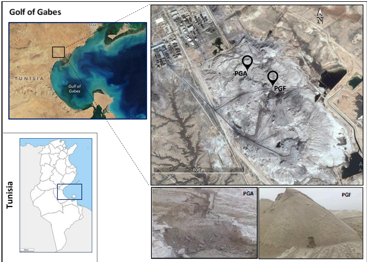
Fig. S1. Study area of the Skhira Phosphogypsum stack, showing the PGA and PGF samples.
