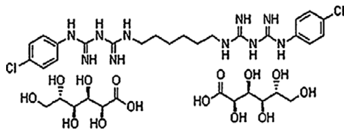
Fig. S1. Structure of chlorhexidine digluconate (CAS: 18472-51-0).
