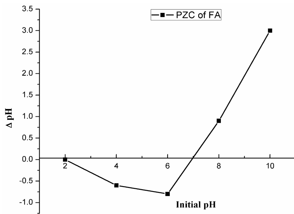
Fig. S3. Point zero charge of fly ash.
