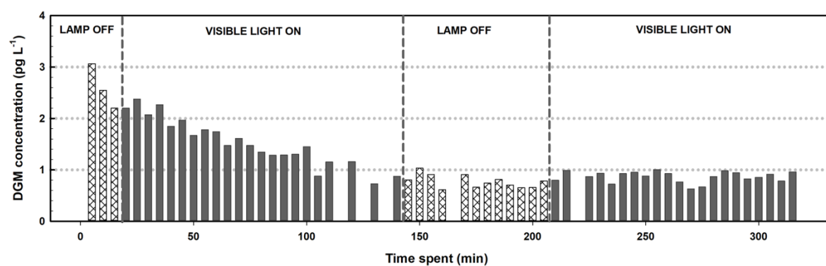
Fig. S1. Dissolved gaseous mercury (DGM) concentration with irradiation of visible light.
